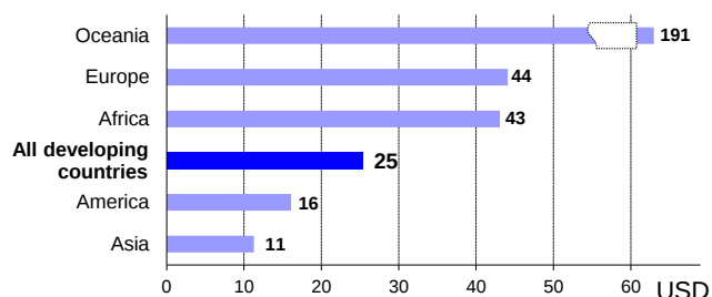
4.1.6. Net ODA receipts per capita in 2014 in USD
