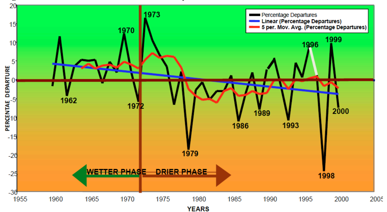
Figure A5. Historical Rainfall Trends in Myanmar
