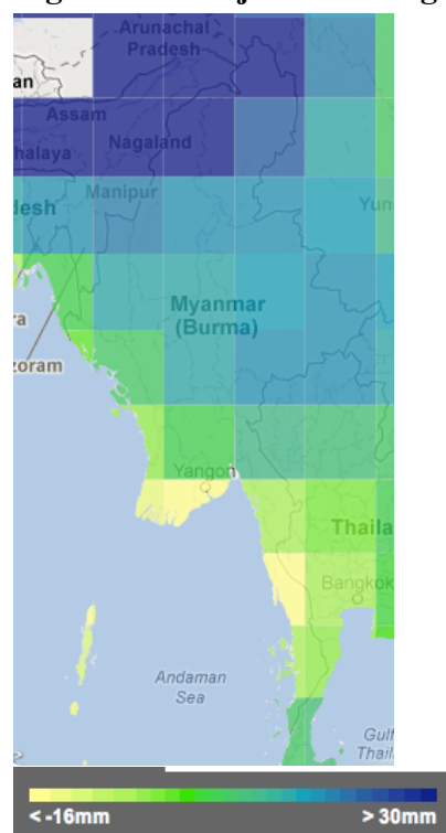
Figure A9. Projected Change in Rainfall for Myanmar for 2080 to 2099
