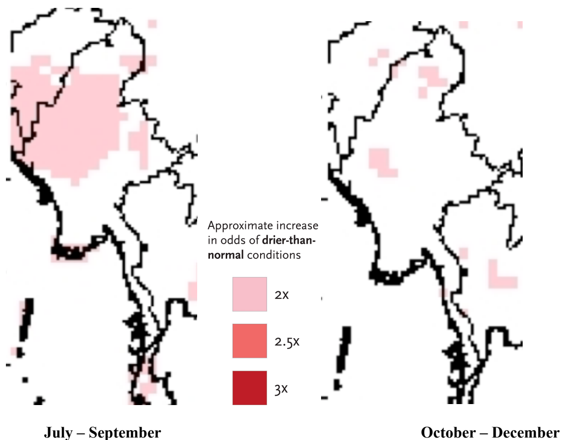
Figure A3. Map Showing Increased Odds of Dry Conditions in Myanmar Due to El Niño Conditions
