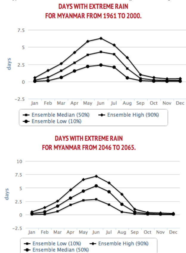
Figure A10. Historical and Projected Days with Extreme Rain in Myanmar
