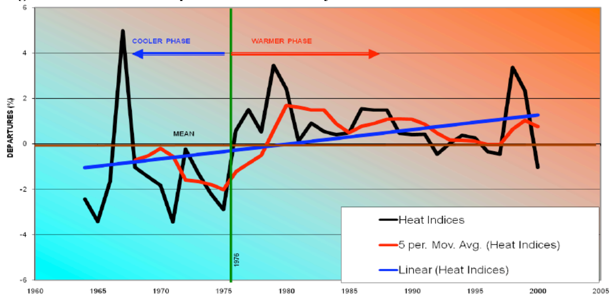
Figure A4. Historical Temperature Trends in Myanmar
