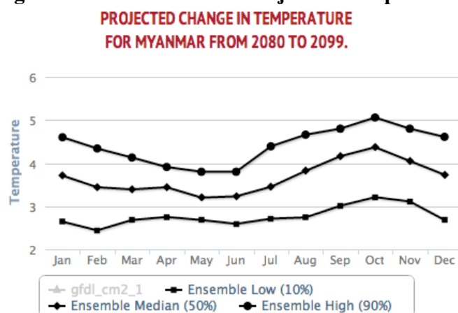
Figure A7. Historical and Projected Temperatures for Myanmar
