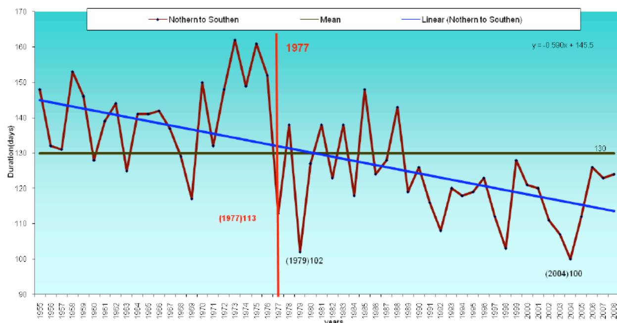
Figure A6. Historical Monsoon Trends in Myanmar
