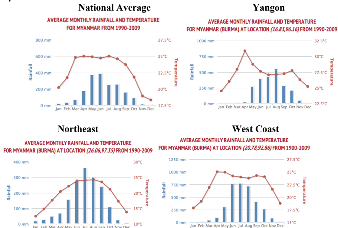
Figure A2. Average Monthly Rainfall and Temperatures for Different Regions of Myanmar
