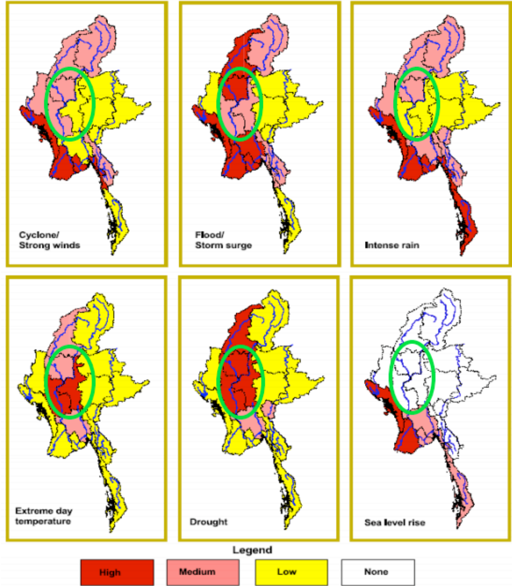
Figure A11. Distribution of Projected Climate Change-related Disaster Risks
